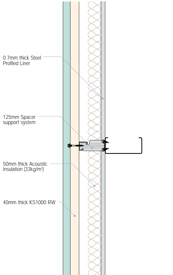
9W - KS1000 RW(40) - Insulated Trapezoidal Wall Panel
